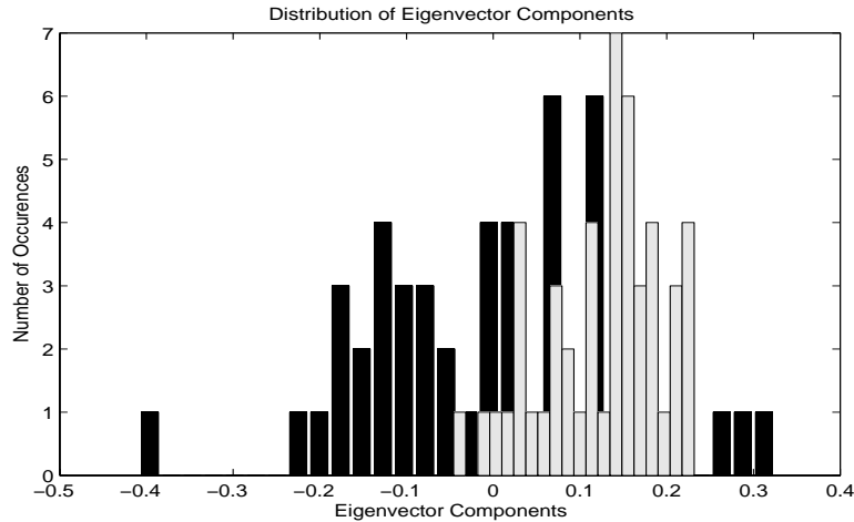
Fig. 3. Comparison of Eigenvector Components, largest Eigenvector (Grey), Eigenvector from the bulk (Black)
