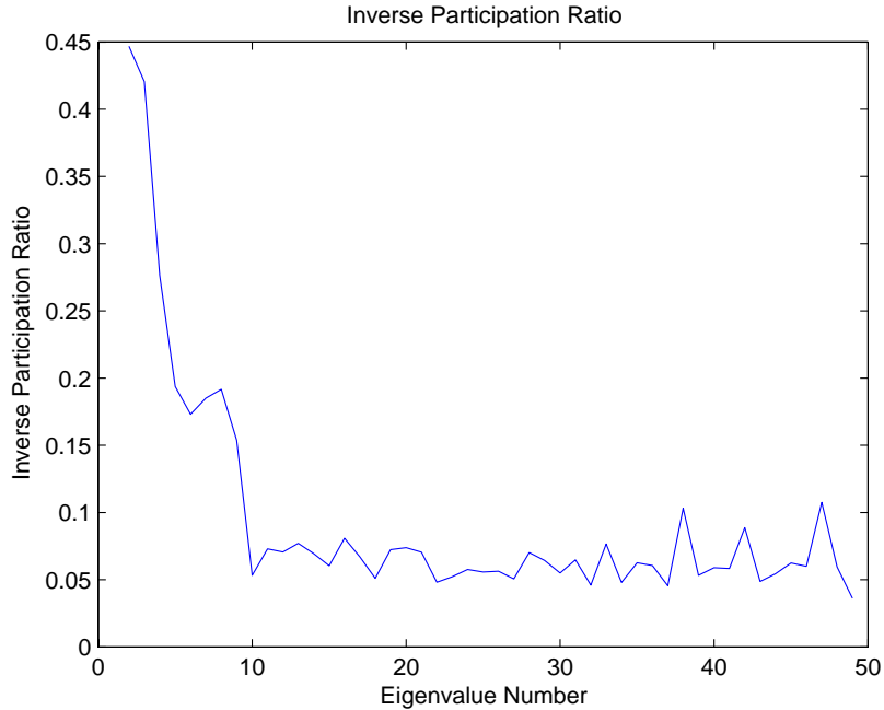
Fig. 10. Inverse Participation Ratio
