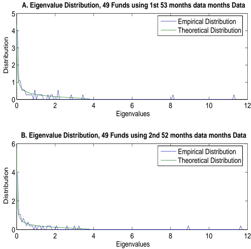
Fig. 2. Bootstrapped spectral distribution for consecutive periods.
