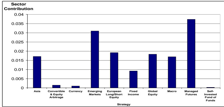
Fig. 7. Strategy Contribution, largest eigenvalue
