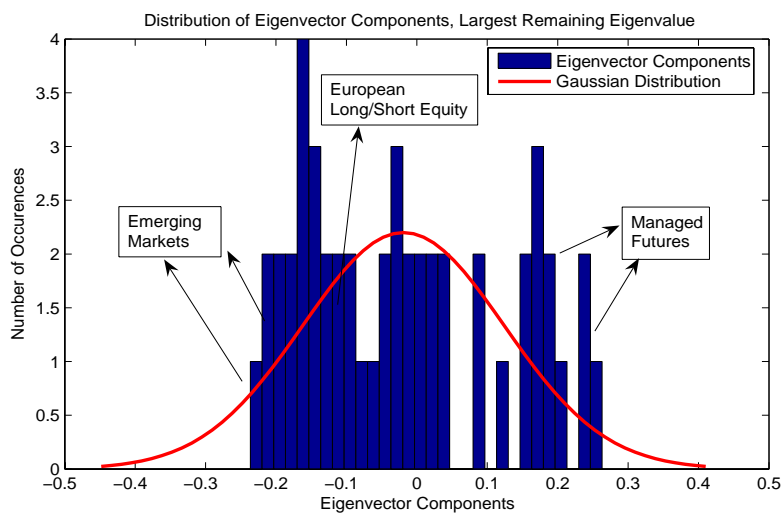
Fig. 5. Distribution of eigenvector components, largest remaining eigenvalue
