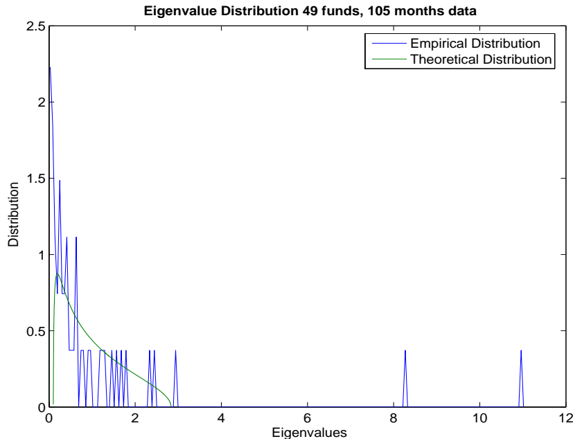
Fig. 1. Spectral Distribution for equally weighted Hedge Fund correlation matrix
